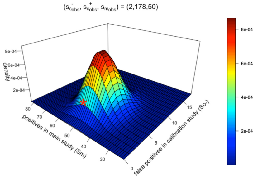
Fig. 1. Density f(\mathbf{S}|H_0) of test positives \mathbf{S} = (S_c^-, S_c^+, S_m) conditional on H_0 of Eq. (5), and with fixed S_c^+ = 178 (its observed sample value) to ease visualization. The observed values (s_{c,obs}^-, s_{m,obs}) = (2, 50) are marked with an asterisk. To test H_0 we need to calculate some kind of “p-value” for the observed point. In our construction, we simply test whether the density at the observed values exceeds an appropriately chosen threshold (see Section 3.2).
