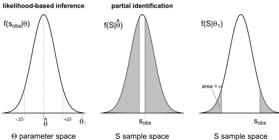
Fig. 2. Illustration of main difference between standard methods of inference, and the partial identification method in this paper. Left: In standard methods, inference is typically based on the likelihood f(s_{\text{obs}}|\theta) as a function over \Theta , and around some mode \hat{\theta} . Parameter values with low likelihood, such as \theta_1 , are not included in the confidence set. Middle & right: In our method, inference is based on the entire distribution function f(s|\theta) over the statistic parameter space, \mathbb{S} . As such, \hat{\theta} will usually be in the confidence set (middle plot). Moreover, \theta_1 will also be in the confidence set if f(s_{\text{obs}}|\theta_1) is high relative to the rest of f(s|\theta_1) even when f(s_{\text{obs}}|\theta_1) is small relative to the mode f(s_{\text{obs}}|\hat{\theta}) (right plot).
