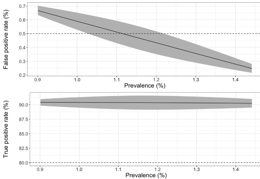
Fig. 10. The MCMC-based 95% confidence set, \hat{\theta} , produced by Procedure 1 of Chen et al. (2018).
