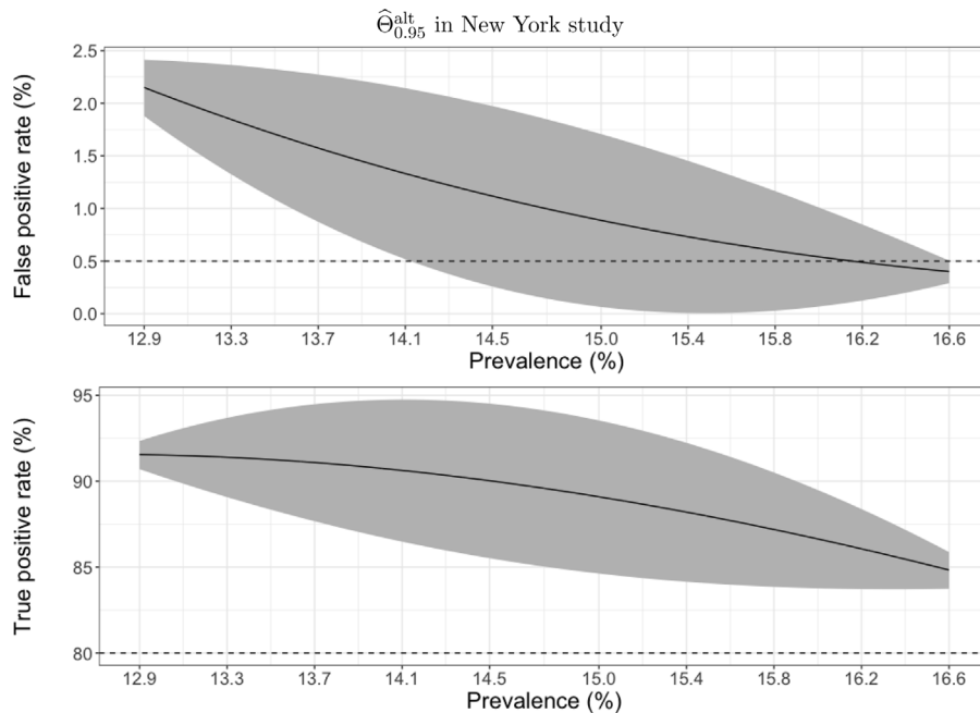
Fig. 5. Visualization of confidence set, \hat{\Theta}_{0.95}^{\text{alt}} , for New York State study. We see that this study gives strong evidence for prevalence in the range 13%–16.6%.
