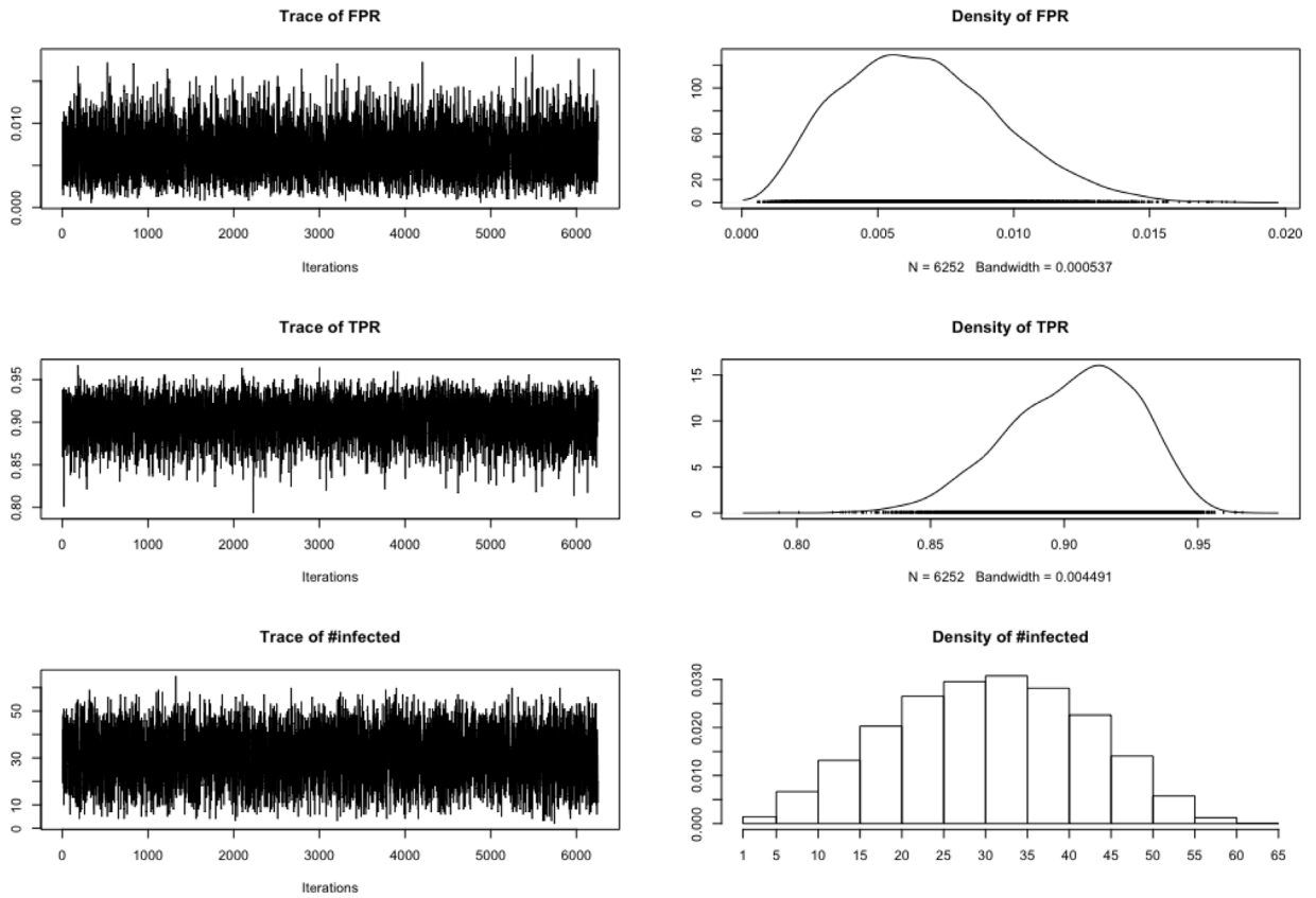
Fig. 9. Mixing plots for the MCMC chain used to construct the 95% confidence set described in Section 4.3.3.
