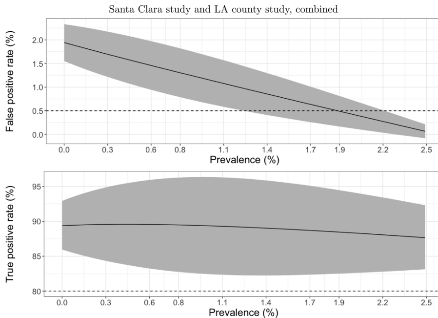
Fig. 8. 95% confidence set from likelihood ratio test-based procedure of Section 4.3.2 for Santa Clara study and LA county study combined.
