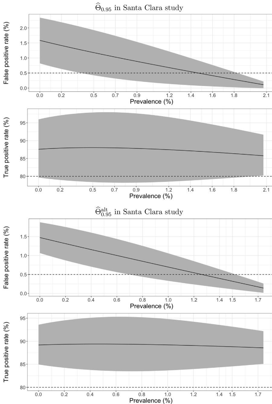
Fig. 3. Confidence sets \hat{\Theta}_{0.95} and \hat{\Theta}_{0.95}^{alt} of the basic and the alternate 95% confidence set construction in Eqs. (8) and (10), respectively, for the Santa Clara study. Each confidence set is broken down to pairwise relationships. All values in a shaded area are in the corresponding confidence set. The horizontal dashed line corresponds to the empirical estimate of the false positive rate ( \hat{p} = 0.5\% ) of the serology test; the dashed line corresponds to the estimate of its true positive rate ( \hat{q} = 80\% ); see Section 4.1 for details.
