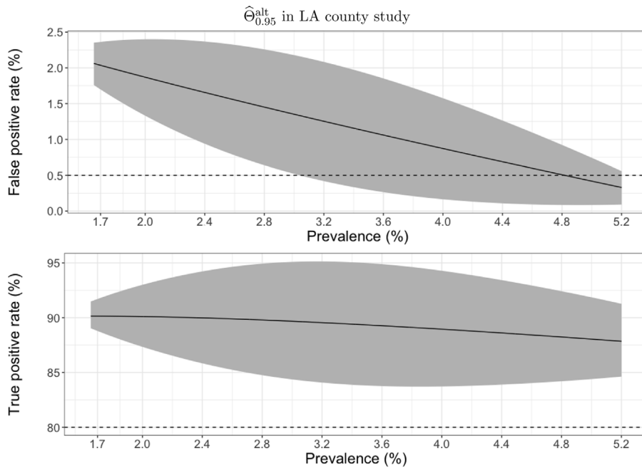
Fig. 4. Visualization of \hat{\Theta}_{0.95}^{\text{alt}} for the LA county study. We see that the evidence for Covid-19 prevalence are stronger than the Santa Clara study. Prevalence is estimated in the range 1.7%–5.2%. This is shortened to 3%–5.2% if we assume a 0.5% false positive rate for the antibody test.
