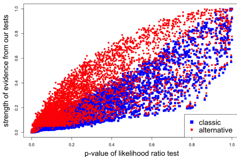
Fig. 6. Relationship between likelihood ratio test and our testing procedures, namely the “classic” construction of Eq. (8), and the alternative construction in Eq. (10).
